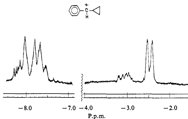
Figure 7. Spectrum in \text{SO}_2\text{-SbF}_5\text{-FSO}_3\text{H} at -60^\circ .
