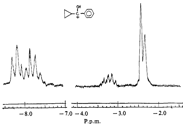
Figure 19. Spectrum in 96% H 2 SO 4 at +40°.
