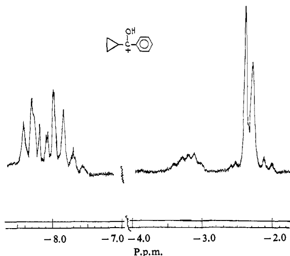
Figure 20. Spectrum in FSO 3 H-SO 2 -SbF 5 at -60°.
