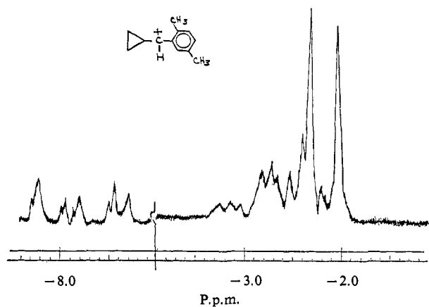
Figure 9. Spectrum in \text{SO}_2\text{-SbF}_5\text{-FSO}_3\text{H} at -60^\circ .
